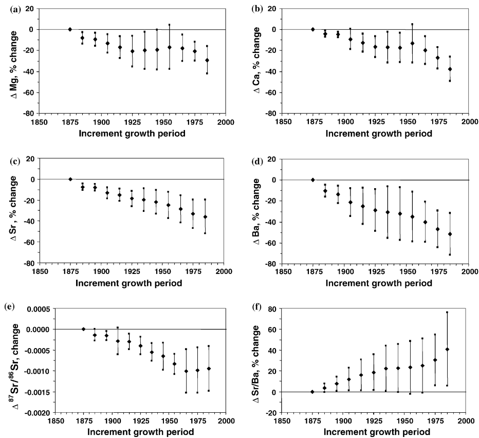
Figure 5. Weighted average (solid diamonds) and standard deviation (lines above and below diamonds) of relative Mg, Ca, Sr and Ba concentrations, \text{}^{87}\text{Sr}/\text{}^{86}\text{Sr} and \text{Sr}/\text{Ba}_{\text{molar}} ratios for spruce stemwood cores having dated wood from 1870 to 1990 (Table 2). Concentrations are plotted in terms of a 'delta' factor that compares the absolute value of the weighted average of increments for each decade to the absolute value for the weighted average for the 1870's decadal increments. The two 3-tree composites are given a three-times weighting compared to the samples from individual trees.
