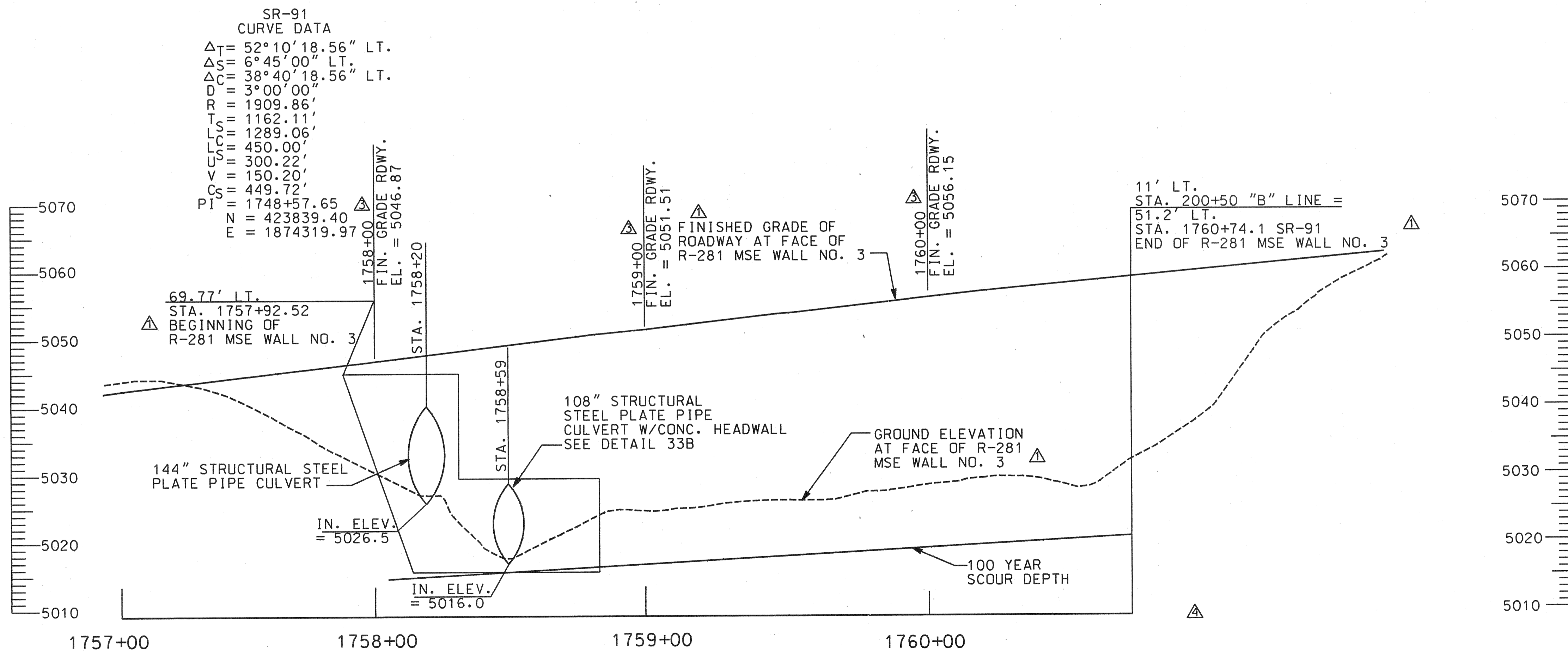
△ R-281 MSE WALL NO. 3 ELEVATION
