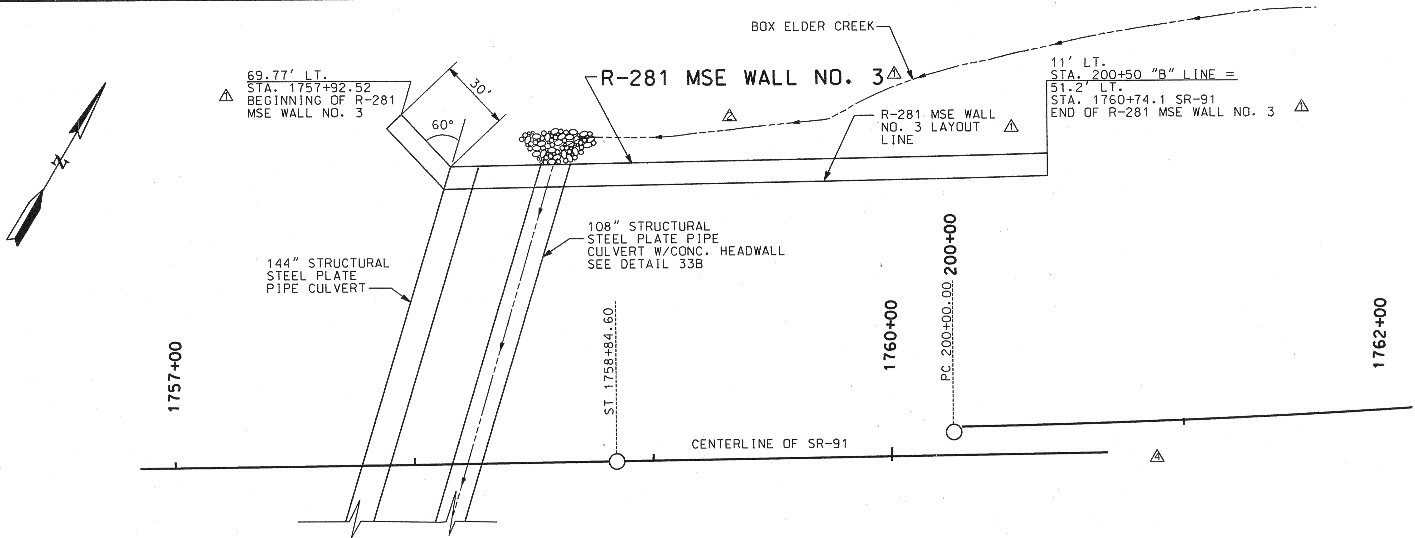
△ LOCATION PLAN R-281 MSE WALL NO. 3
