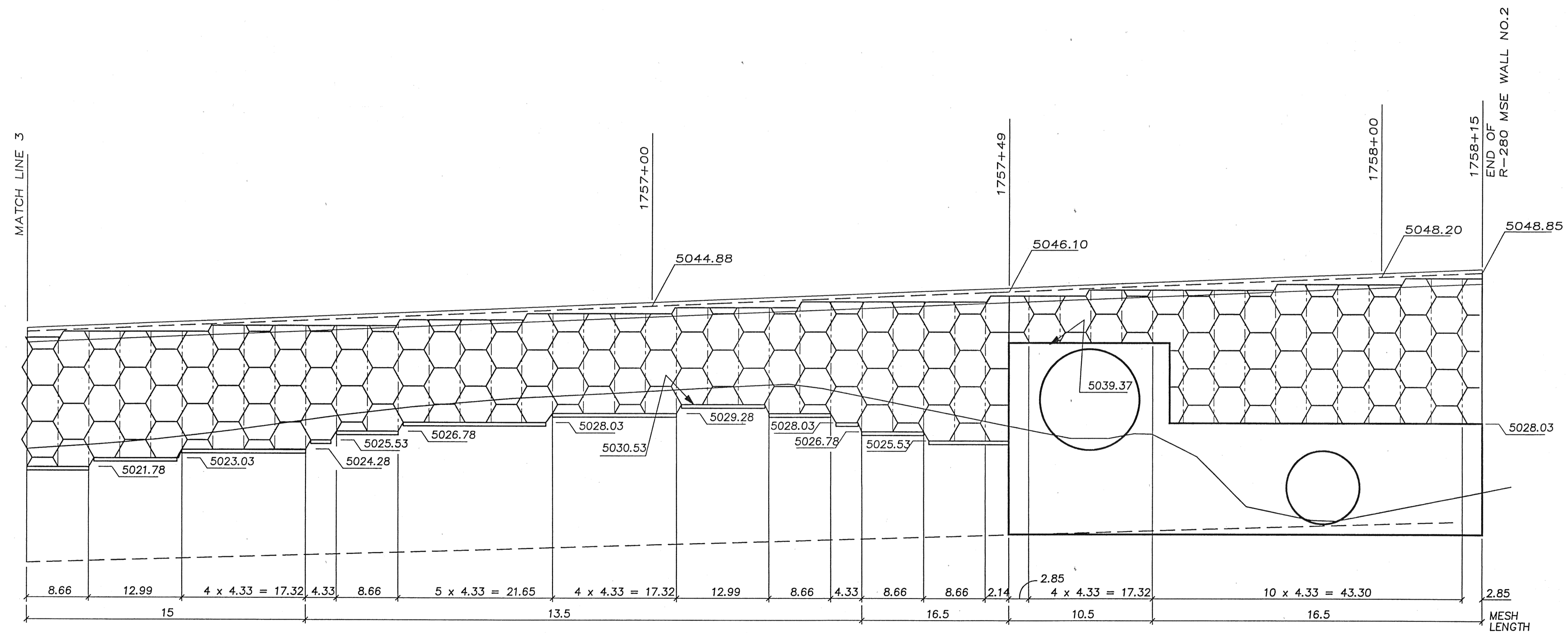
R-280 MSE WALL NO.2 ELEVATION (ELEVATION LOOKING SOUTH) SCALE 1"=10'-0"
