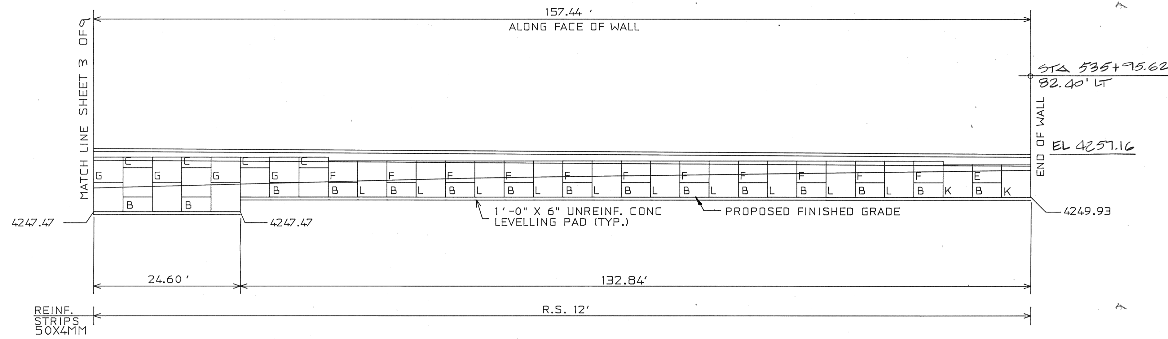
WALL NO.2 WEST WING WALL FRONT FACE ELEVATION
