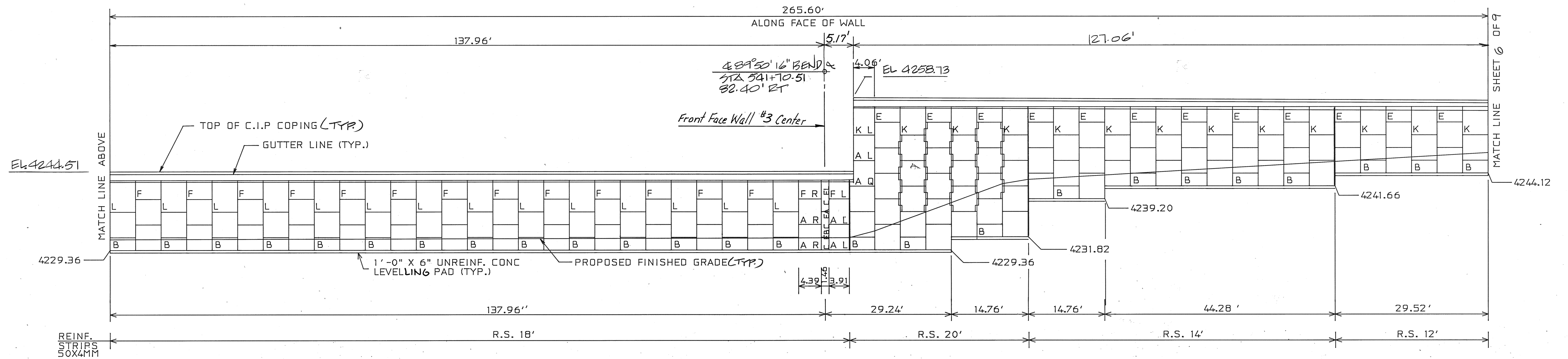
WALL NO.3 EAST FRONT FACE - ELEVATION
