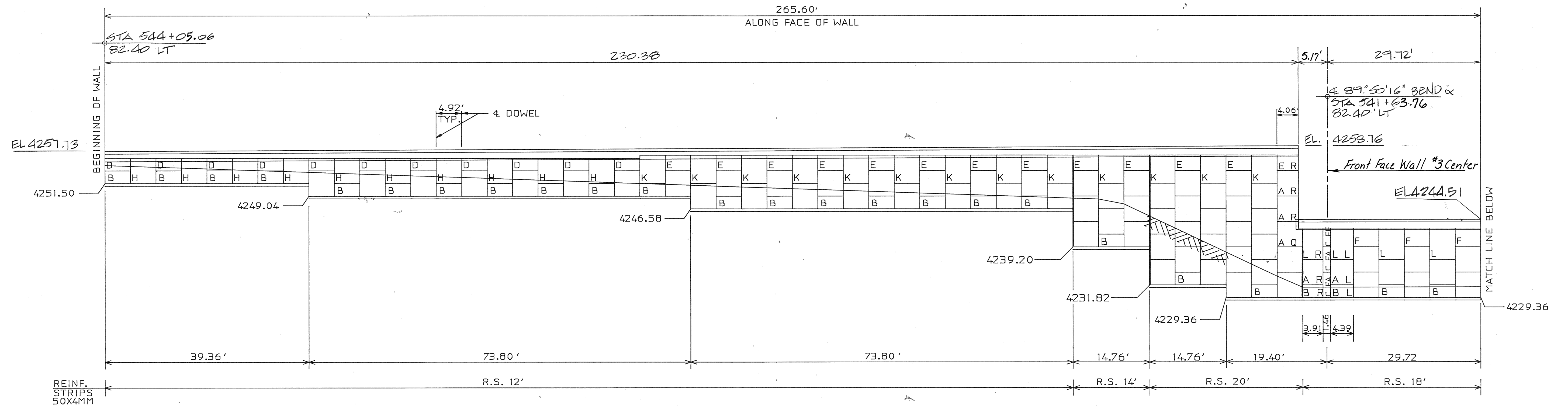
WALL NO.3 WEST FRONT FACE - ELEVATION
