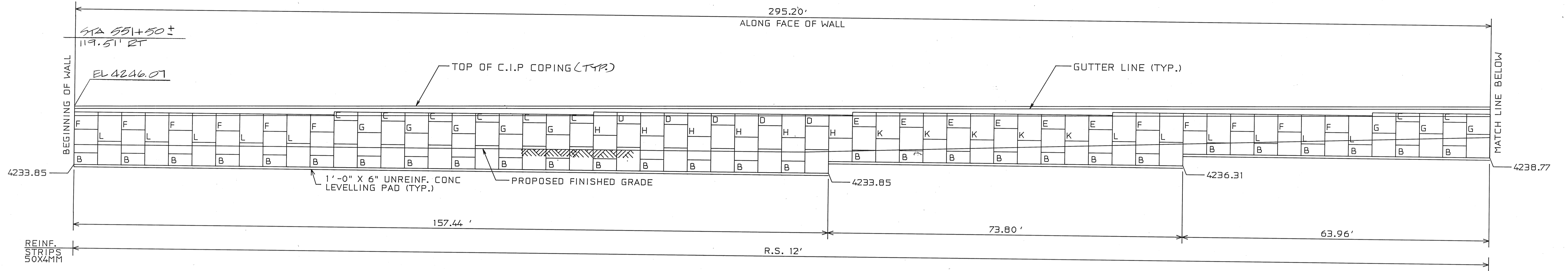
WALL NO. 4 FRONT FACE ELEVATION
