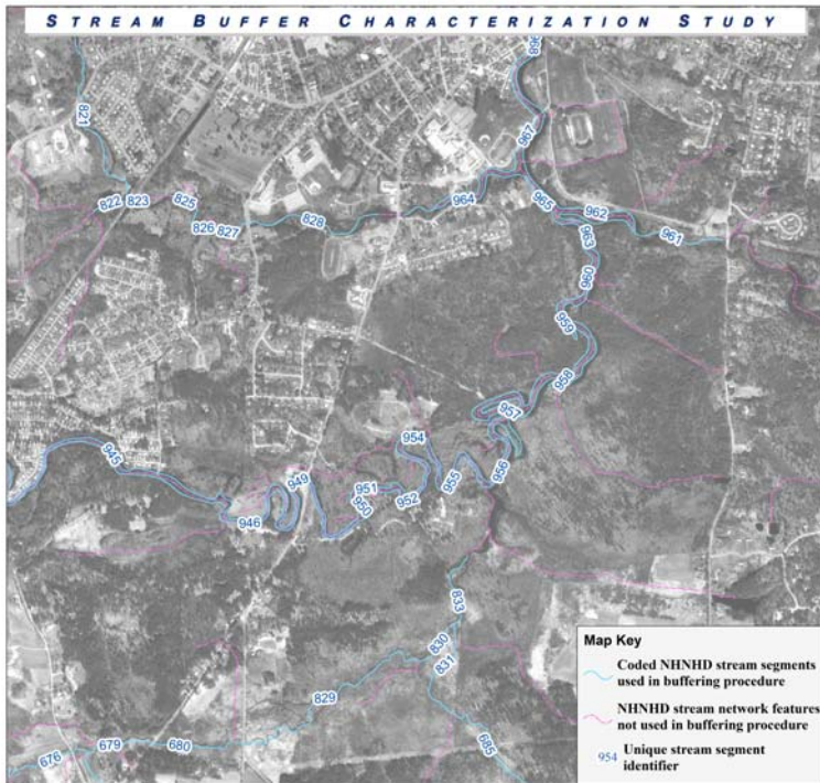
Figure 3. Stream coding based on confluence to confluence segments.
